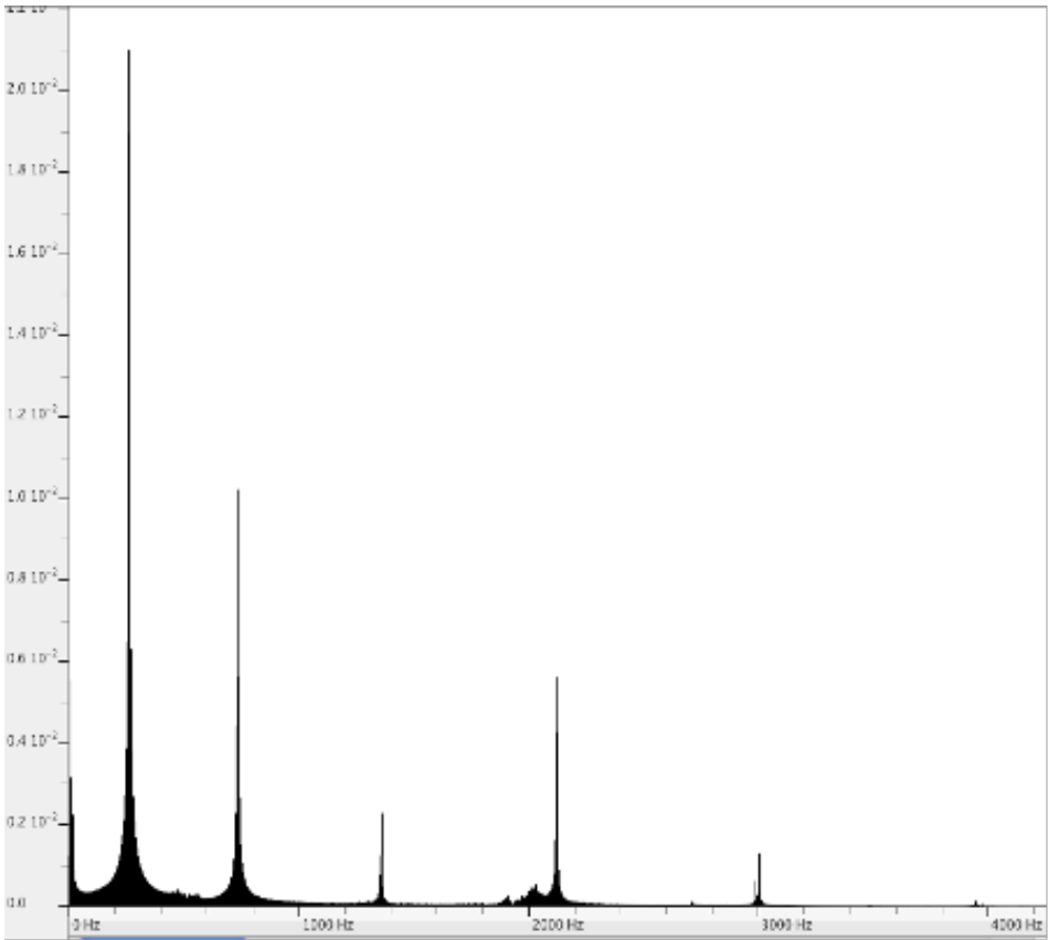
Fig. 3a): Spectrum analysis for sample ‘C4 hard+EQ’
