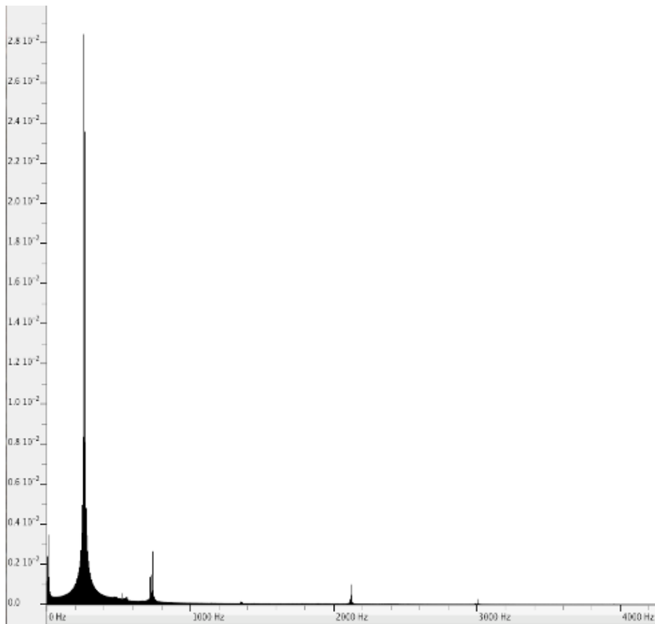
Fig. 3b): Spectrum analysis for sample 'C4 soft + EQ'
