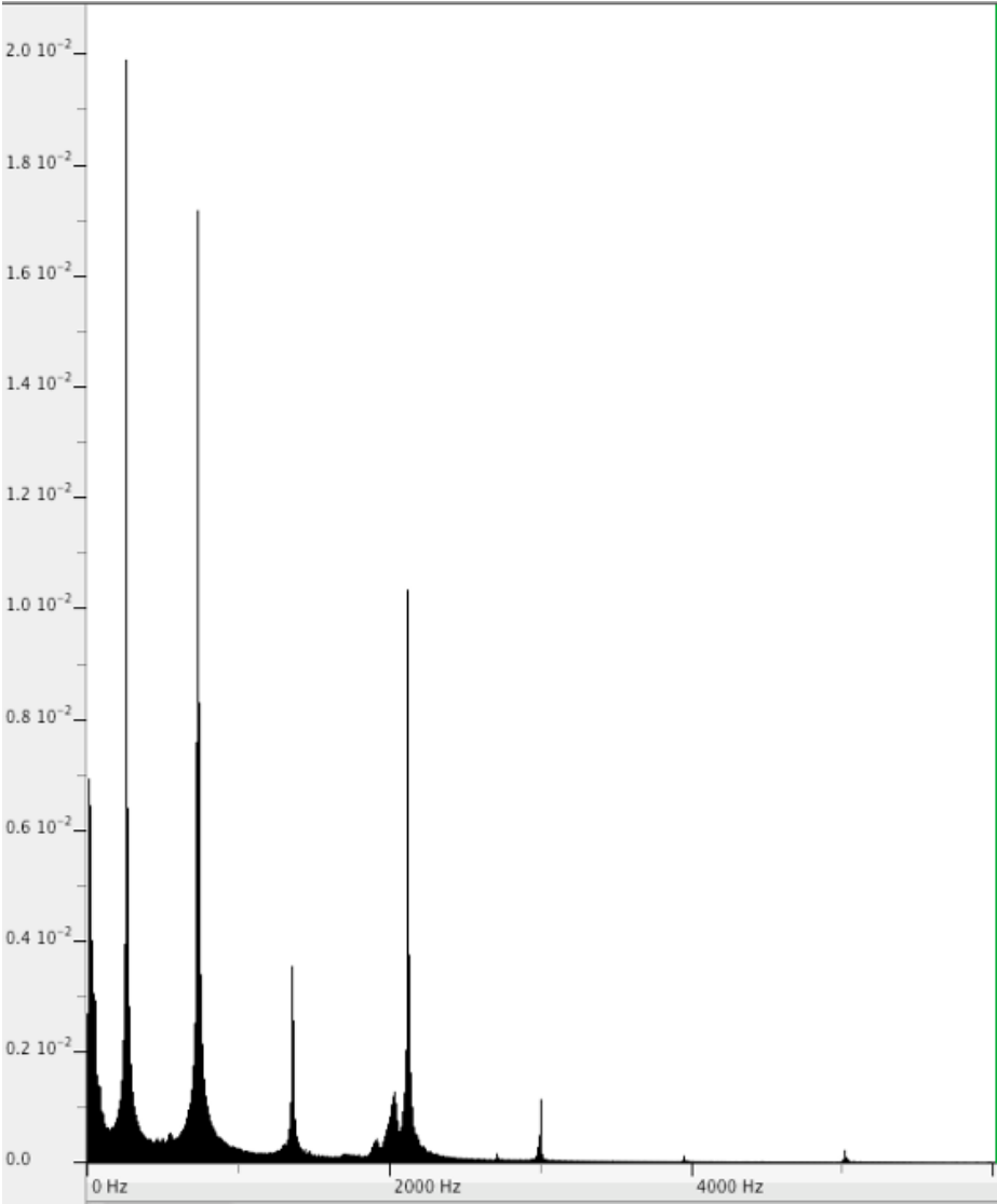
Fig. 2a): Spectrum analysis for sample ‘bowl C4 hard’
