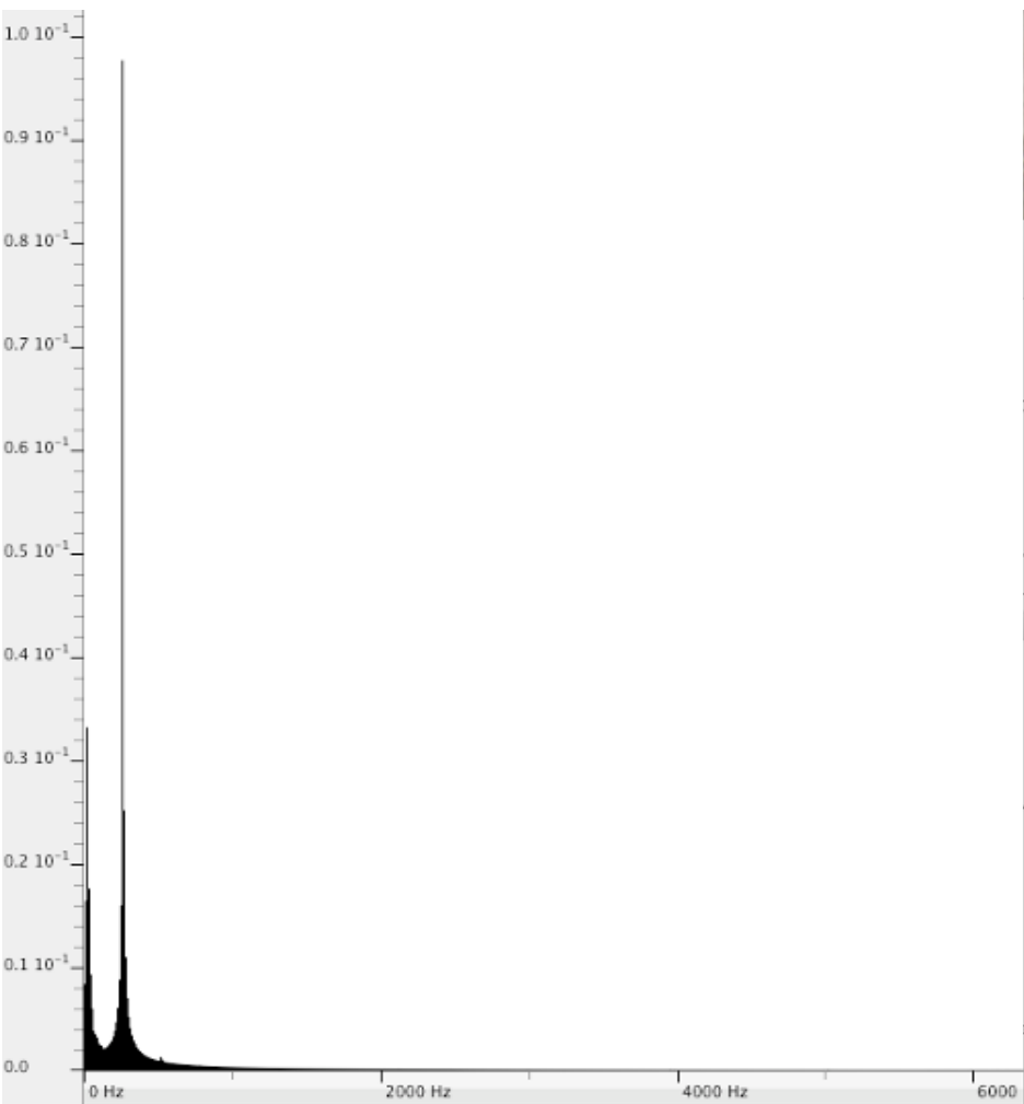
Fig. 2c): Spectrum analysis for sample ‘bowl C4 singing’
